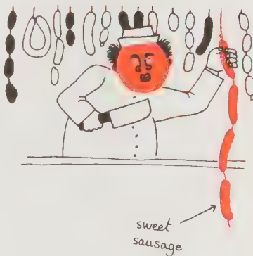
A BUTCHER
