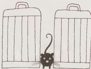
BETWEEN
