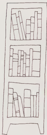
bookshelf
