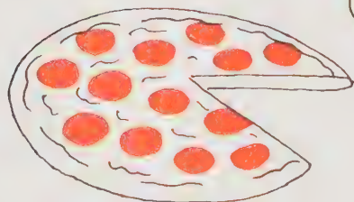
pepperoni pizza
