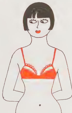
SMALL
