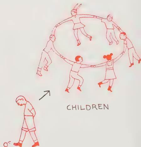
CHILD
