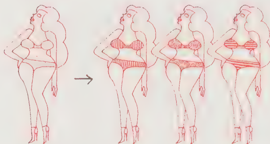
WOMAN
