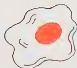
fried egg
