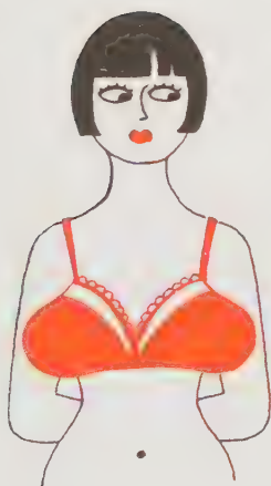
BIG
