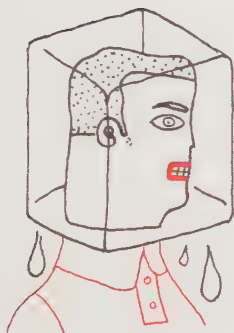
COLD
