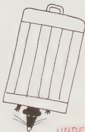
UNDER
