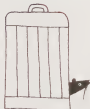
BEHIND
